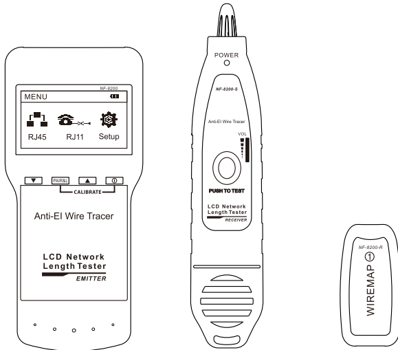
Main tester (NF-8200)
