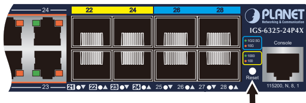
Figure 6-3: IGS-6325-24P4X and IGS-6325-24P4S Reset Button
