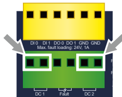
Figure 3-1: 6-contact terminal block connector of IGS-6325-20T4C4X and IGS-6325-20S4C4X
