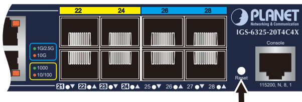
Figure 6-1: IGS-6325-20T4C4X Reset Button
