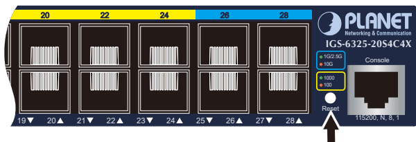
Figure 6-2: IGS-6325-20S4C4X Reset Button
