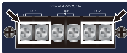
Figure 3-2: 6-contact terminal block connector of IGS-6325-24P4X and IGS-6325-24P4S
