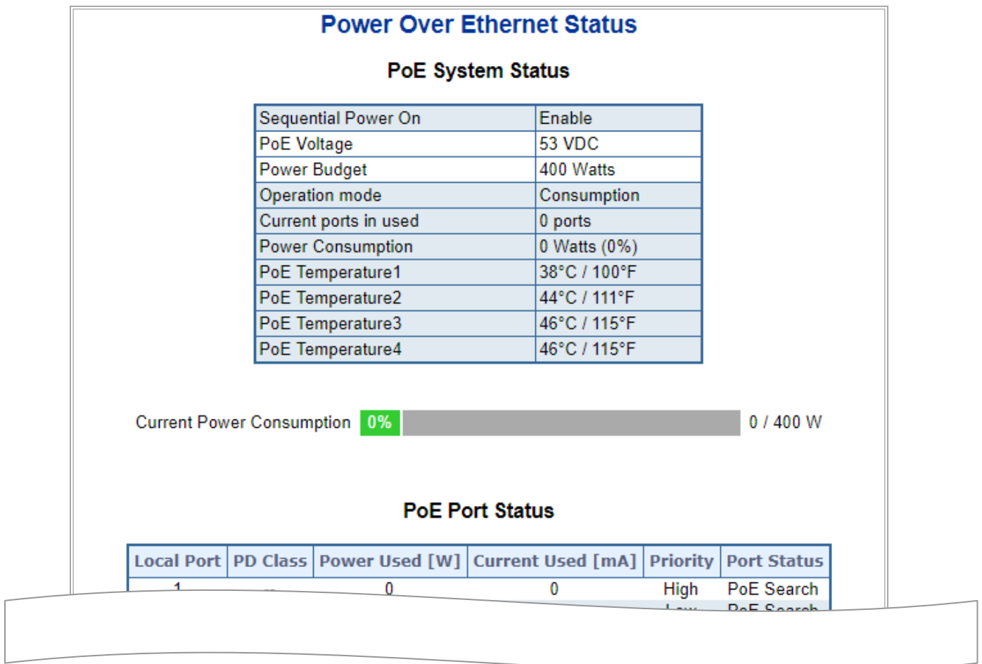
Figure 4-6-1-1: Power over Ethernet Status
