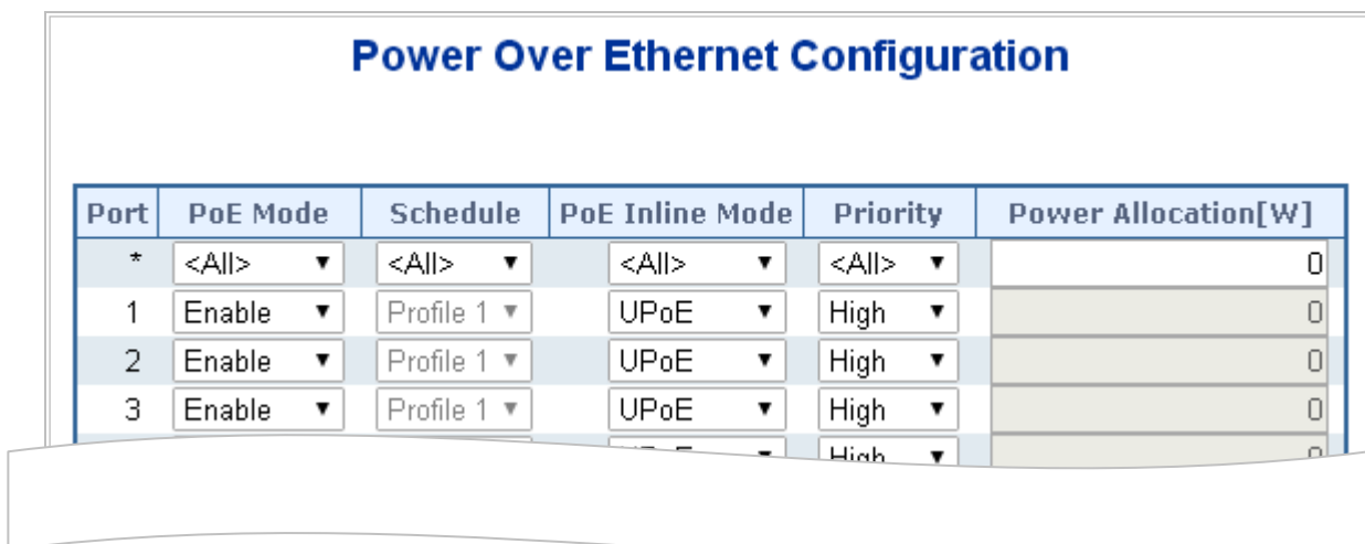
Figure 4-6-1-3: Power over Ethernet Configuration Screenshot
